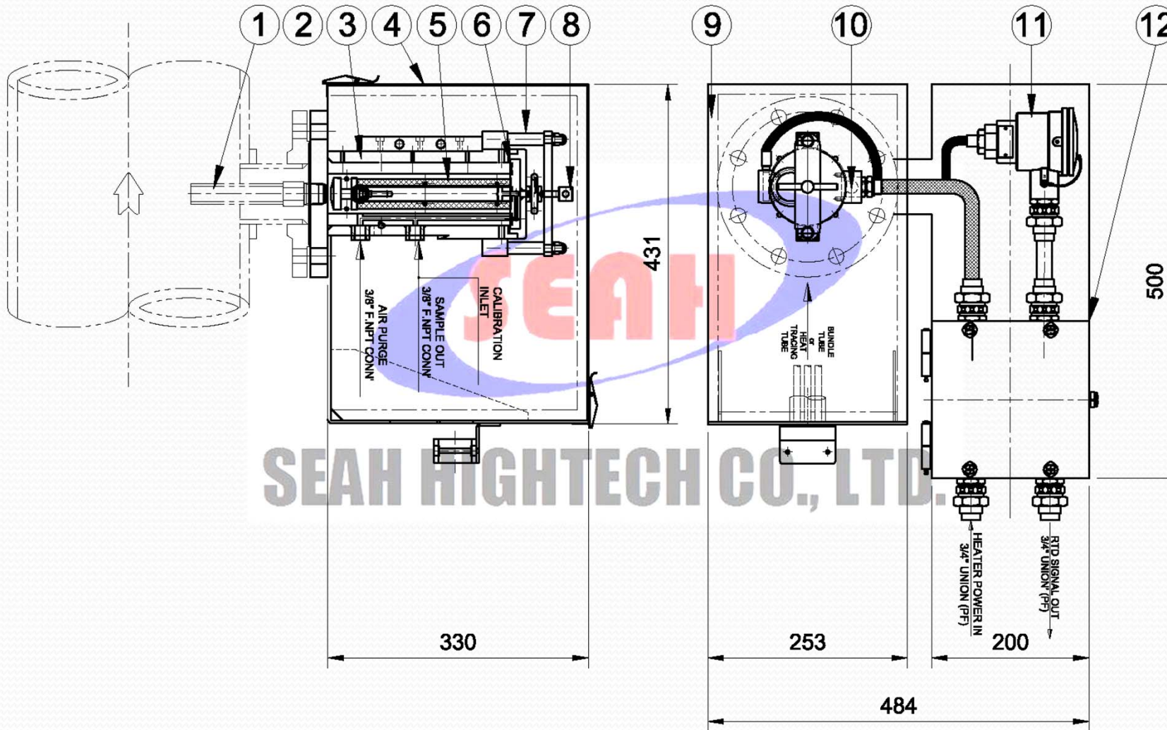
SIDE VIEW
